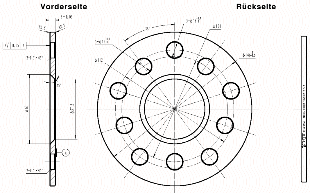
Detail -1-
