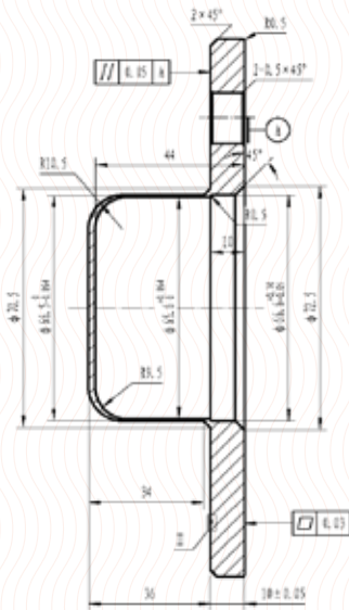
Detail -1-
